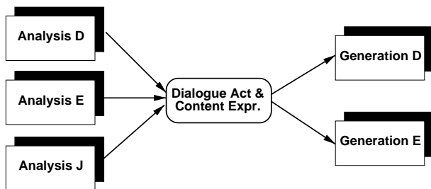
Figure 3: Content expressions as intermediate representation for translation
