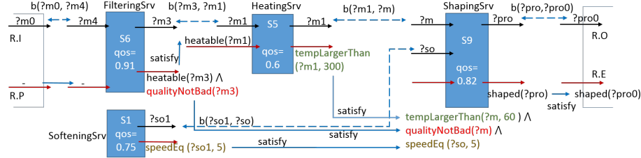
Fig. 1: An example workflow with parameter bindings.
