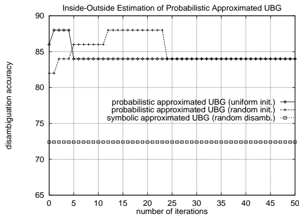
Figure 6: Precision on exact match task in number of training iterations for probabilistic context-free approximations, starting with uniform and random probabilities for the grammar rules. Baseline is the disambiguation accuracy of the symbolic approximated UBG.
