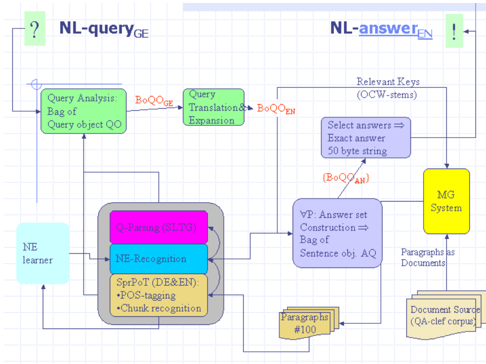
Figure 1: A blueprint of BIQUE’s architecture.
