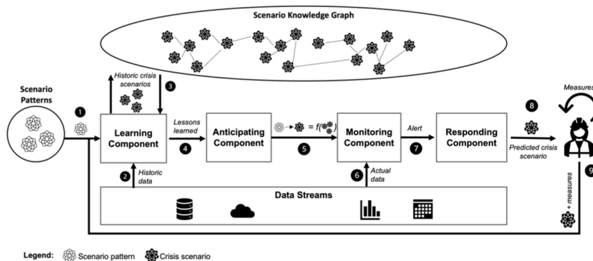
Figure 4: AI-based scenario planning for predicting crisis situations: AISOP module [9]
