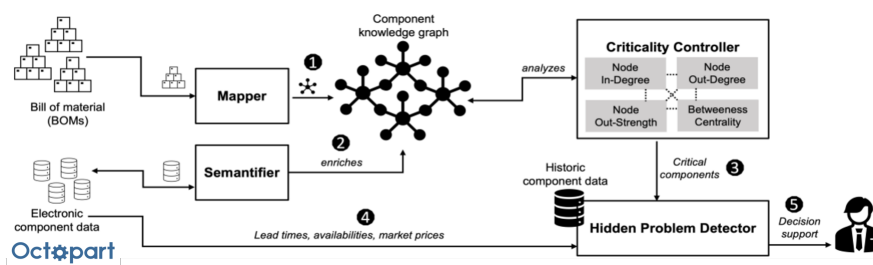
Figure 5: Model for graph-theoretic analysis of component criticality in supply chains: Hidden Problem Detector module [17]
