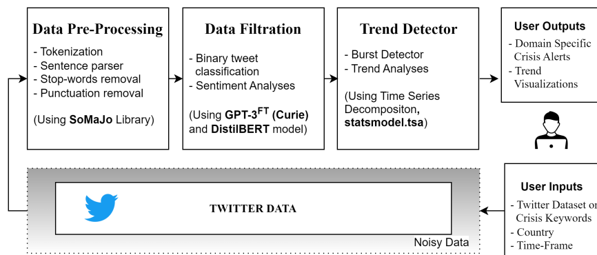
Figure 6: Model for open-domain social signal detection of crisis-related indicators in tweets: Social Signal Observer [21]
