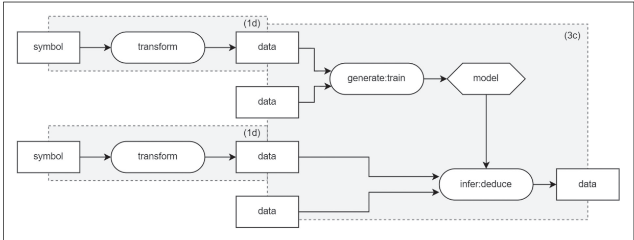
Figure 8. Synergised LLMs and KGs for reasoning. KG: knowledge graph; LLM: large language model.
