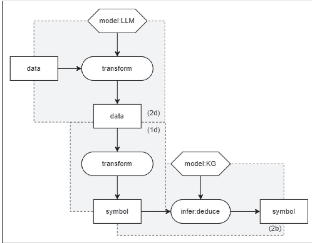
Figure 7. LLM-augmented KGs during inference. KG: knowledge graph; LLM: large language model.
