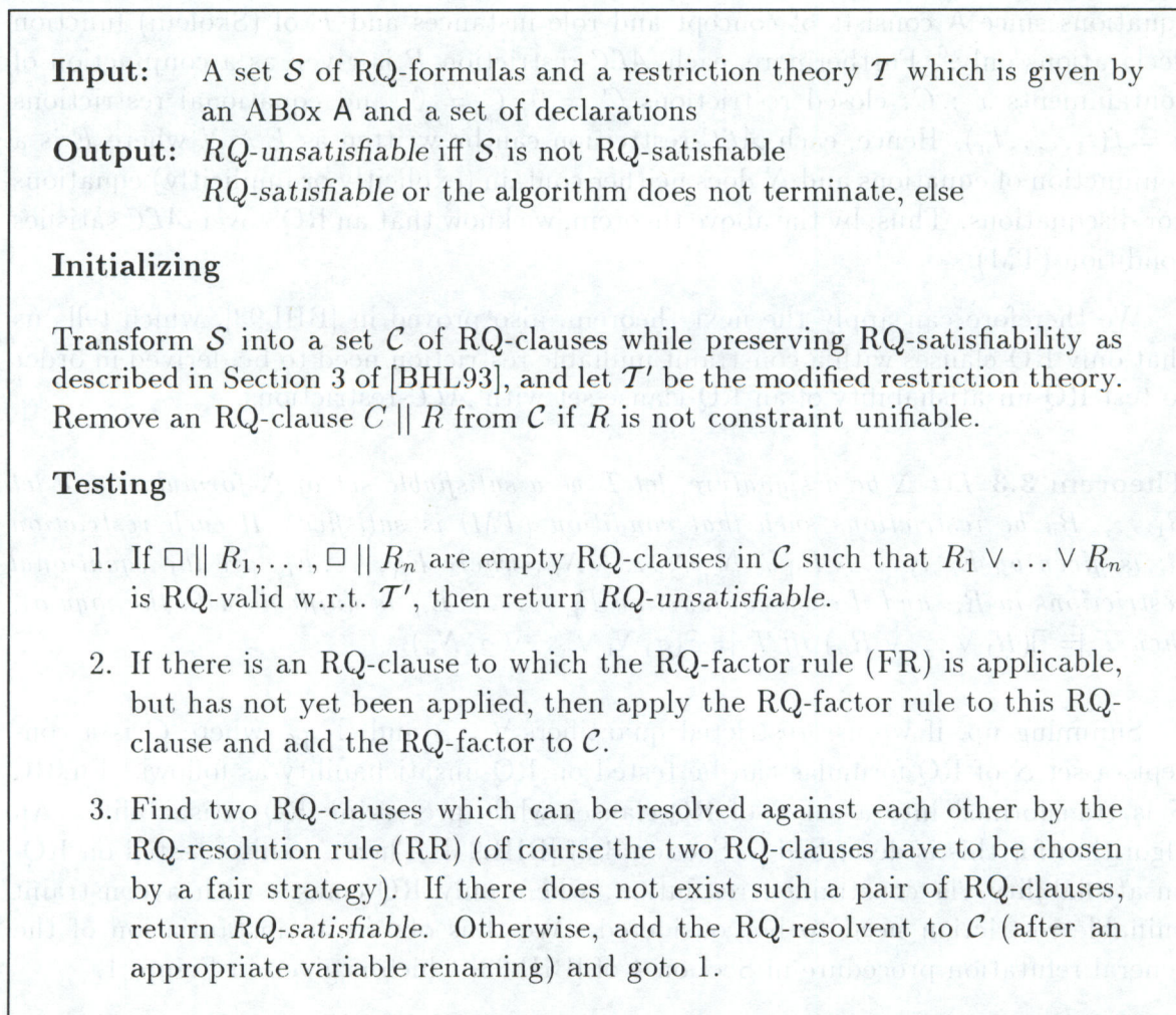
Figure 1: The refutation procedure.
