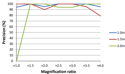
Figure 3. Relationship between magnification ratio and precision of character recognition.
