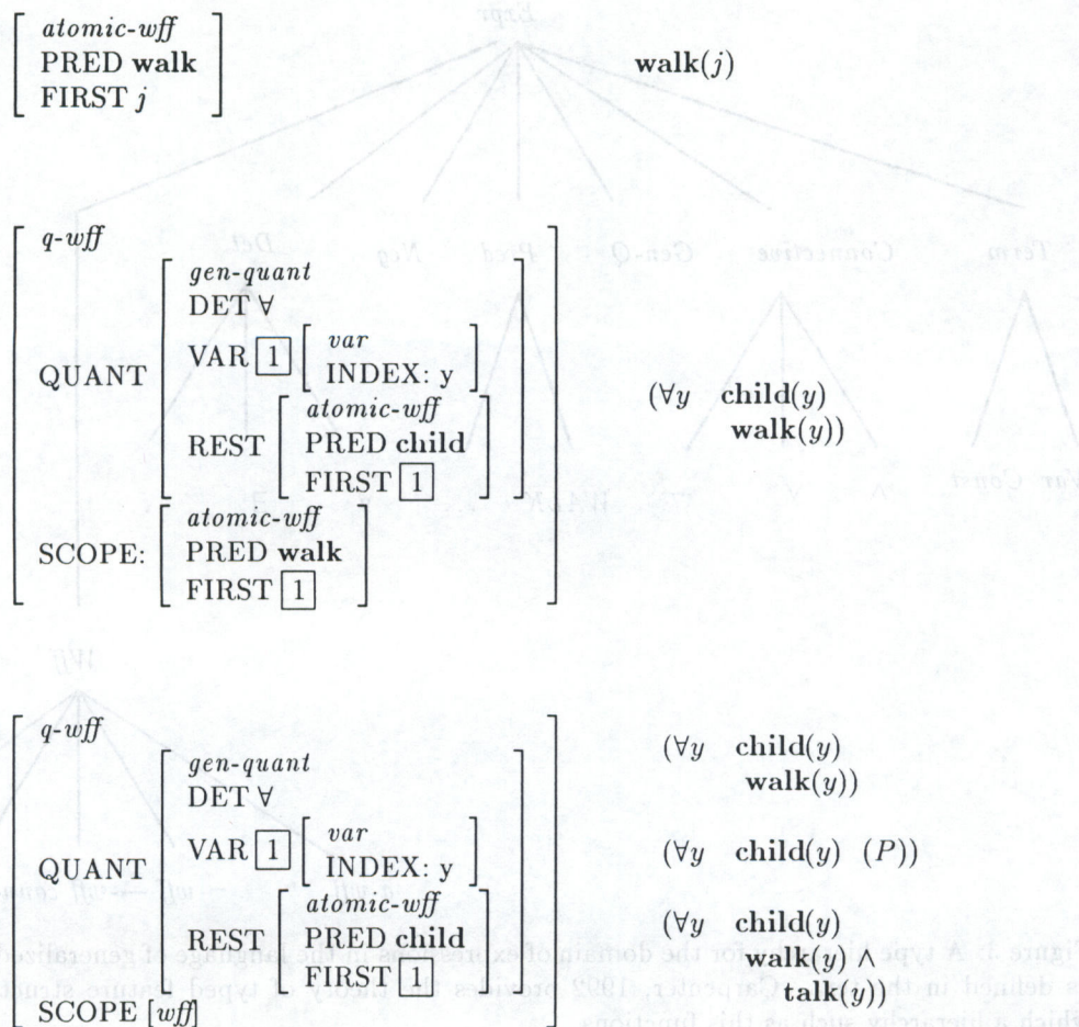
Figure 4: Feature structure descriptions used as metalinguistic descriptors of expressions in LGQ. Note the use of underspecification in the last example.
