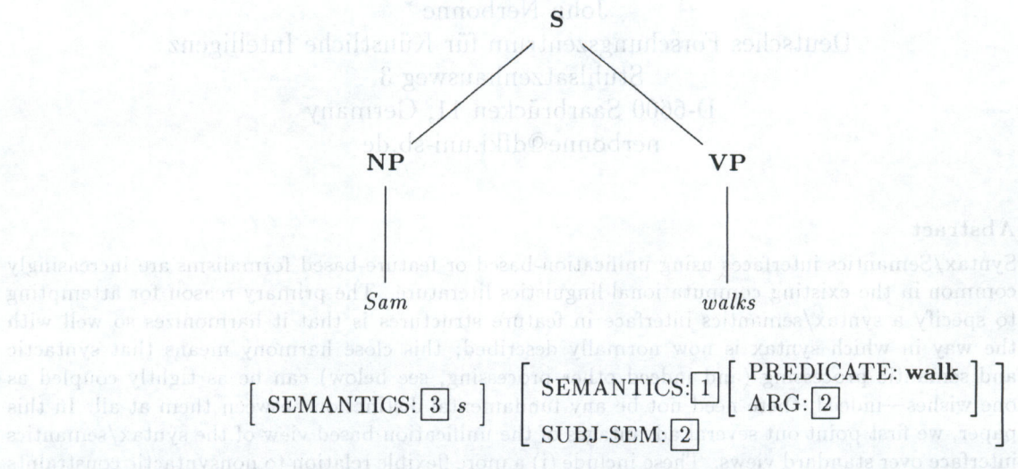
Figure 1: A sketch of the semantic derivation of Sam walks , walk ( s ) as this would proceed using unification. Unification applies to syntactic and semantic representations alike, eliminating the need to compute these in distinct processes, and unification is employed to bind variables to argument positions, eliminating the need for (a great deal of) \beta -reduction as used in schemes derived from Montague and the lambda calculus.
