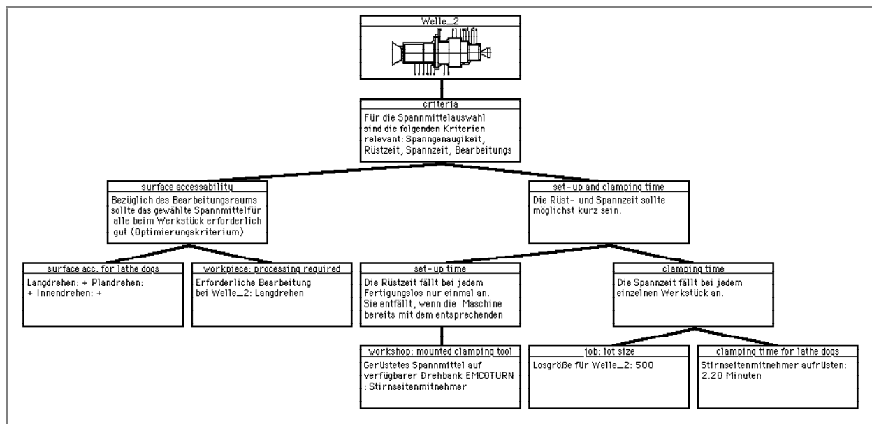
Figure 3.2: Part of an explanation tree justifying the use of a lathe dog for manufacturing the workpiece "Welle_2." 2
