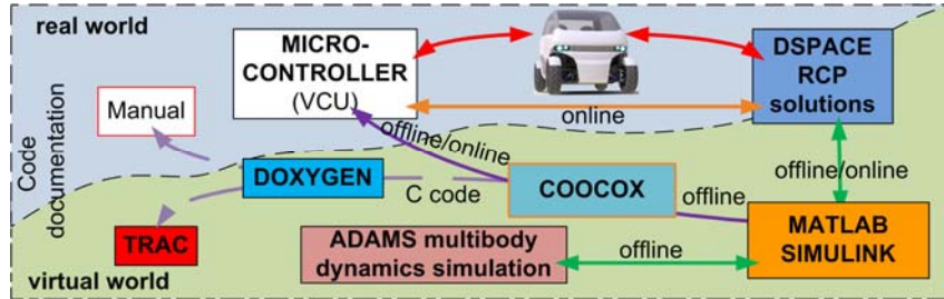
Fig. 2. Tools used within the framework divided into virtual (simulation) and real (hardware)
