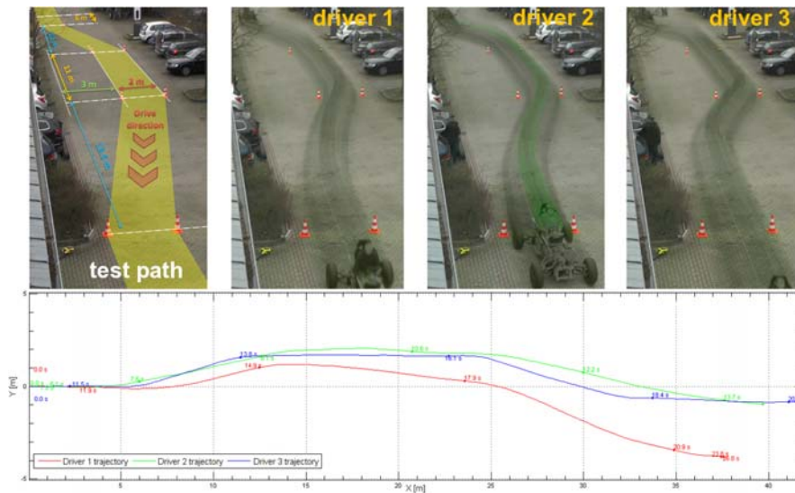
Fig. 6. Lane change experiments for three drivers and corresponding trajectories from simulation replay.
