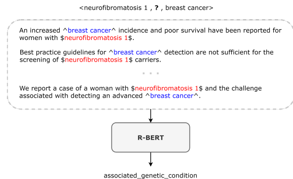
Figure 1: Example of a distantly supervised bag of sentences for a knowledge base tuple ( neurofibromatosis 1, breast cancer ) with special order sensitive entity markers to capture the position and the latent relation direction with BERT for predicting the missing relation.
