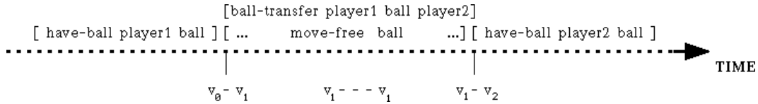
Figure 4: Corresponding interval-based representation
