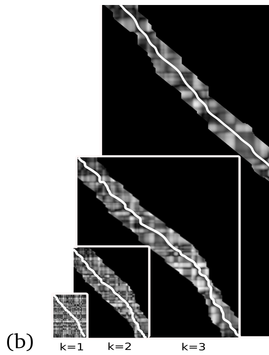
Figure 2: (a) The Adaptive DTW algorithm. (b) At each iteration, as the Warp path is projected onto the higher resolution, the slope constraint of the DTW algorithm is incremented
